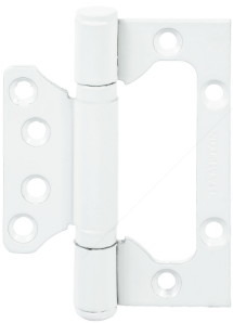
ONE LEAF HINGE ES IR HPT OL 4x3x2,8MM 2BB WHITE
